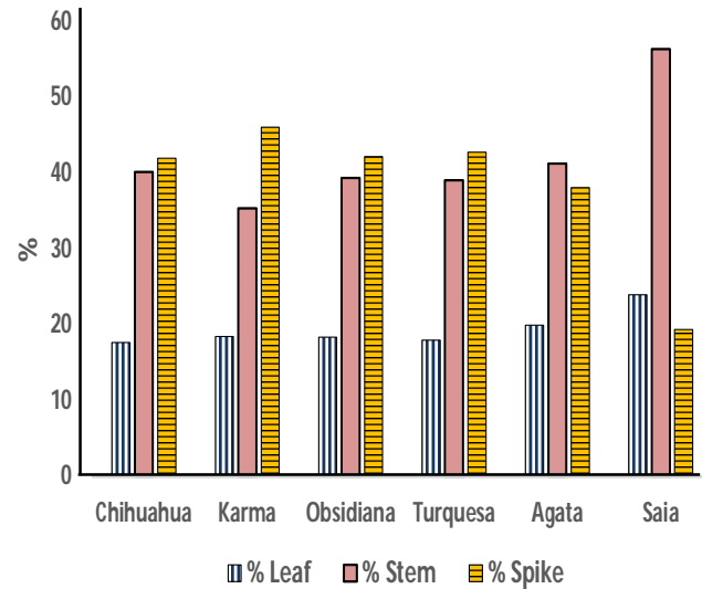
Figure 2. Proportion of yield components of oats varieties
